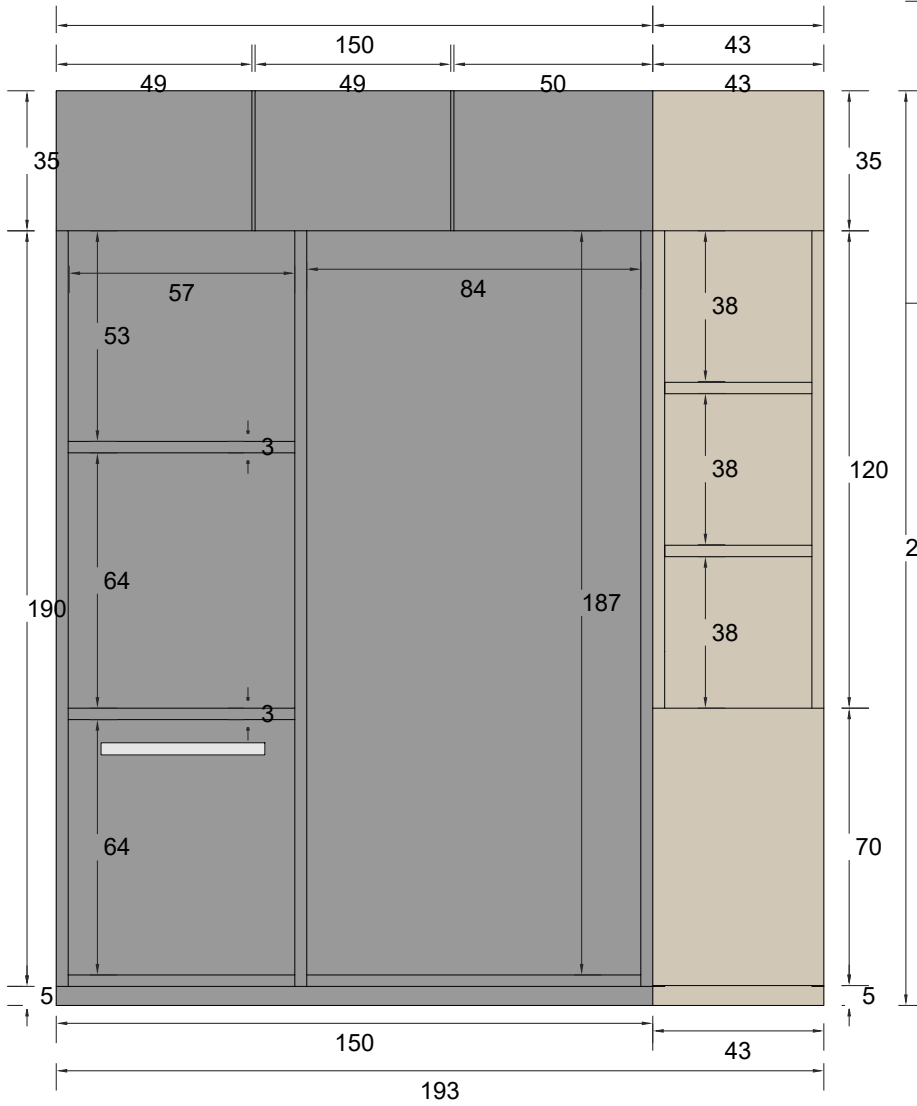
FRIDGE AREA FRONT ELEVATION
